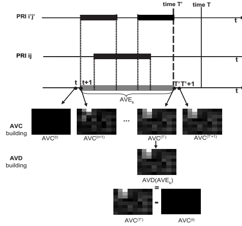
Figure 3. Building process of the AVC and AVD matrices: considering overlapping PRI's relative to audio and video subspaces i and j (on the bottom) and i' and j' (on the top), that form the k -th AVE, we can see how the AVC is calculated until the time step T . The dashed line corresponds to the final step T' of the AVE. After that time step, no AV association holds among any subspaces, therefore AVC matrix remains unchanged and the AVD matrix relative to the AVE k is calculated.
