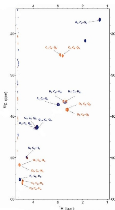
Fig. 3 Aliphatic regions of 1 H- 13 C HSQC NMR spectra of the Ac-F 1 C 2 G 3 D 4 G 5 A 6 N 7 D 8 C 9 G 10 -Am peptide, 2.5 mM, pH 6.3, T 298 K, in the absence (orange) and in the presence (blue) of 0.1 equivalents of Mn(II).
