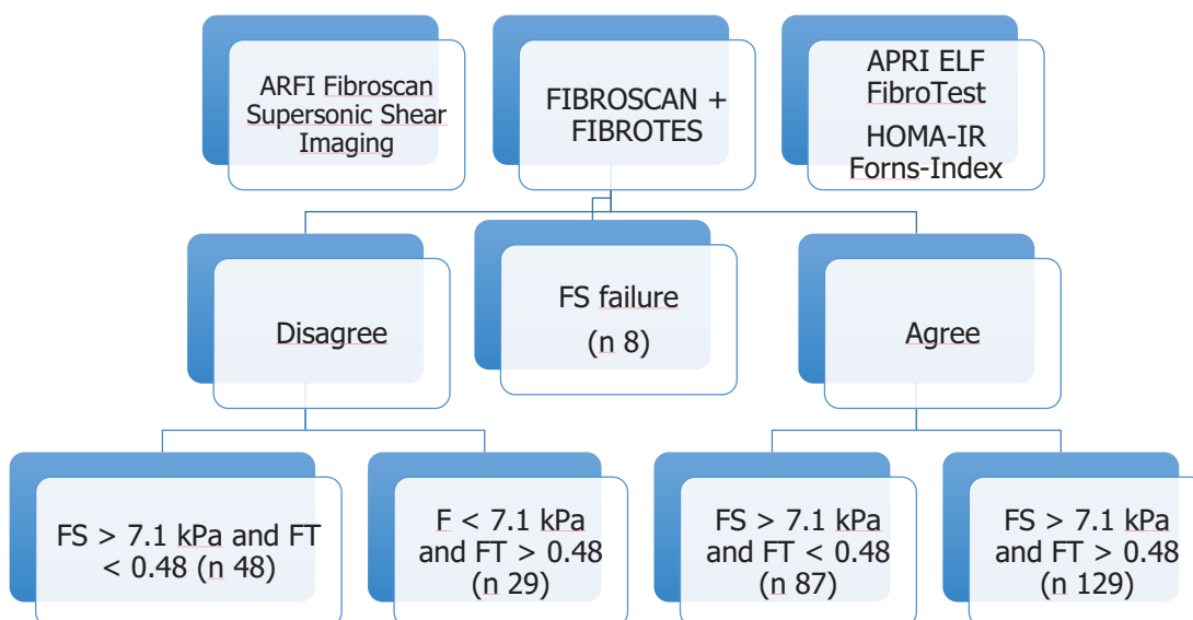
Figure 2: Castera/Bordeaux algorithm
