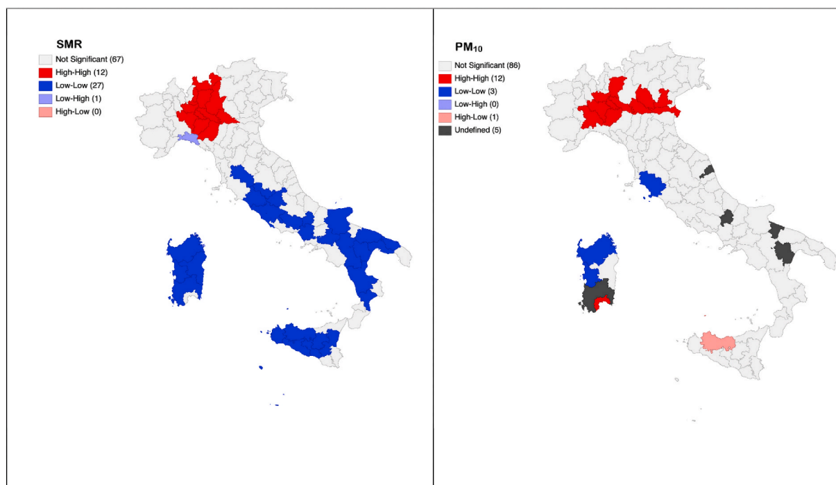
Fig. 4. Analysis of Spatial Autocorrelation – LISA. SMR and PM_{10} (color should be used). (For interpretation of the references to color in this figure legend, the reader is referred to the Web version of this article.)
