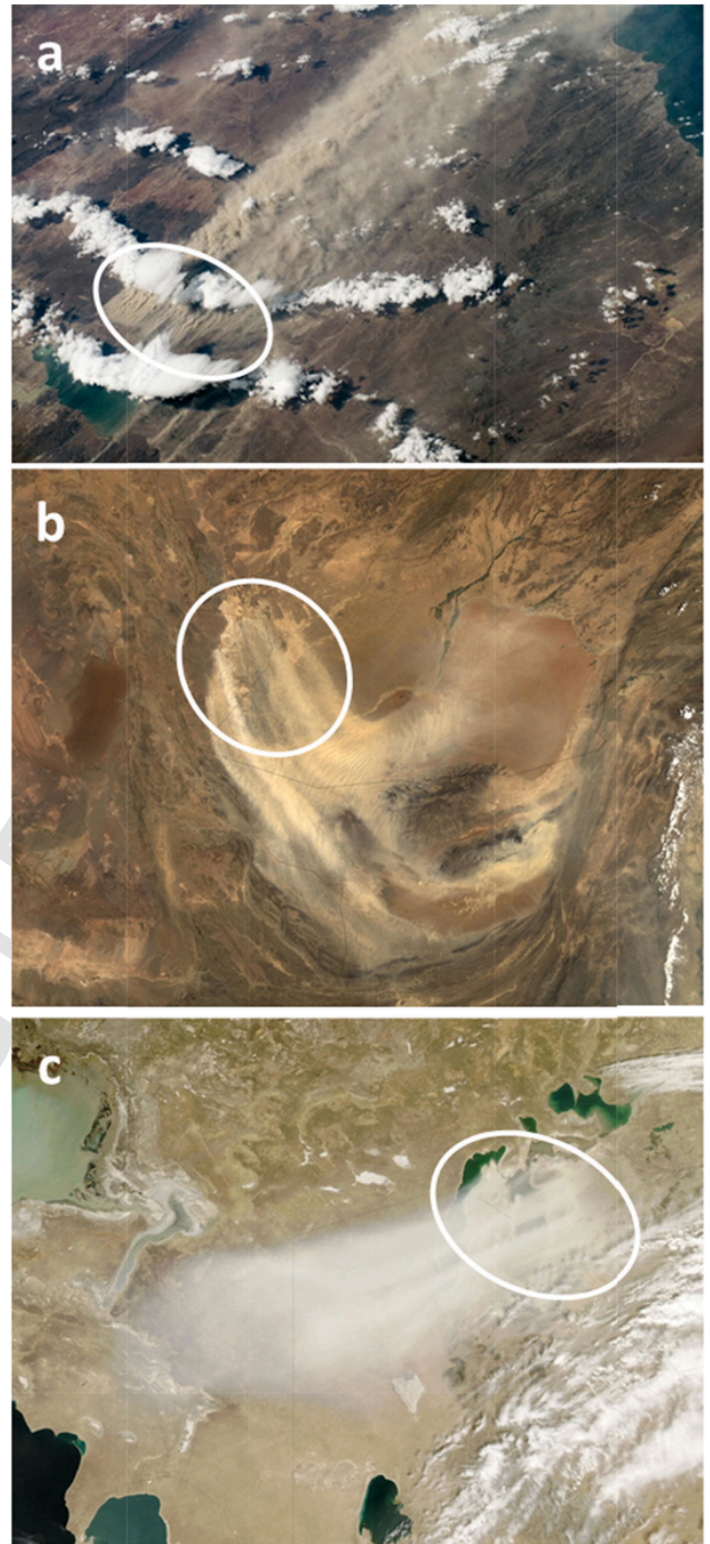
Fig. 2. (a) A dust storm passing over Patagonia region of southern Argentina on March 7, 2020. The main dust source is Lago Colhué Huapi ( -45.5 Lat, -68.7 Long), a shallow lake adjacent to the deeper Lago Musters. In the photograph the lake is largely obscured by dust and clouds. NASA Image courtesy, astronaut photograph ISS062-E-85589 taken by a member of the Expedition 62 crew. https://earthobservatory.nasa.gov/images/146681/patagonian-dust-streamers (b) Dust plumes originating from the almost completely dry bed of the Hamoun Lakes ( 30.8 Lat, 61.6 Long), in the Sistan Region of Iran, cover the arid terrains of southern Afghanistan (top), Iran (left), and Pakistan (bottom right), as shown by true color images by the Moderate Resolution Imaging Spectroradiometer (MODIS) aboard NASA's Terra satellite, on August 20, 2003. NASA Image courtesy Jacques Desclouetres, MODIS Land Rapid Response Team at NASA GSFC https://earthobservatory.nasa.gov
