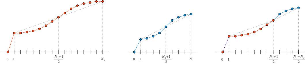
Figure 25: construction of the test function \bar{v} .
