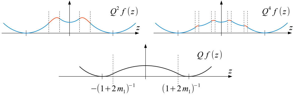
Figure 15: The function z \mapsto Q^M f(z) for different values of M and the limit function.
