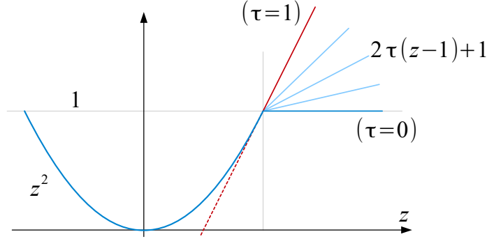
Figure 13: example of convex-affine non-convex potentials.
