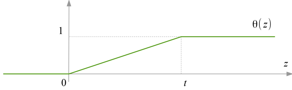
Figure 4: Graph of the phase function \theta(z) for the function f^t in Example 3.13.
