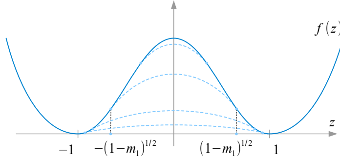
Figure 2: the function Q_{\mathbf{m}}f in Remark 2.30 with f(z) = (1 - z^2)^2 for different values of m_1 < 1 .
