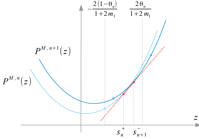
Figure 32: Envelope of two consecutive functions P^{M,n}(z)
