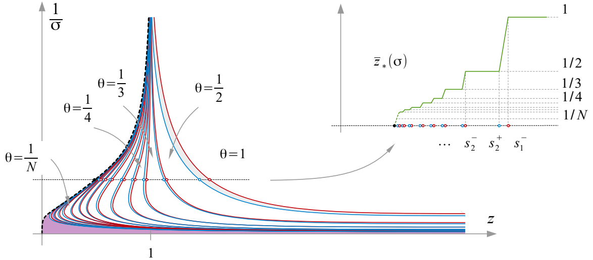
Figure 30: representation of \theta in the z-\frac{1}{\sigma} plane and a cross section at fixed \sigma .
