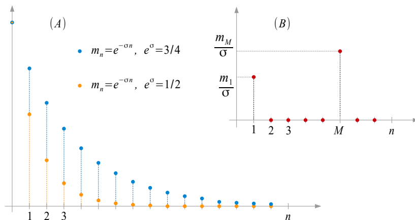
Figure 1: representation of exponential and concentrated kernels.
