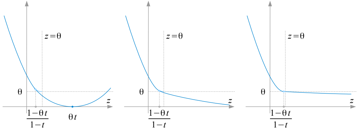
Figure 5: Graph of Q_0 f^t(\theta, z) with \theta fixed and increasing values of t .
