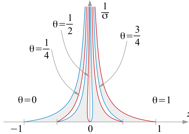
Figure 19: Representation of constancy sets of \theta in the z - \frac{1}{\sigma} plane ( M = 4 ).
