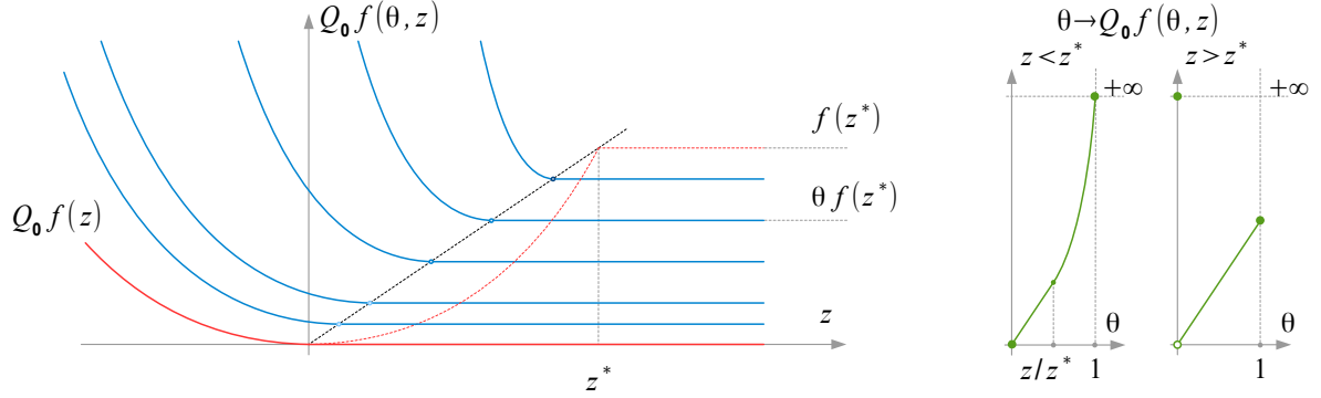
Figure 6: (a) Q_0 f(\theta, z) for a truncated convex potential and (b) \theta \mapsto Q_0 f(\theta, z) for different values of z .
