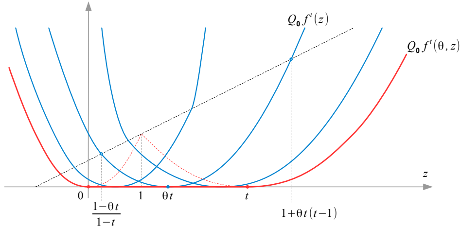
Figure 3: Graph of Q_0 f^t(\theta, z) for different values of \theta .
