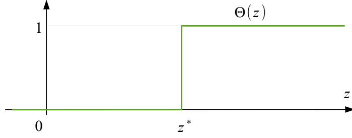
Figure 7: the phase multifunction \Theta(z) in the convex case.
