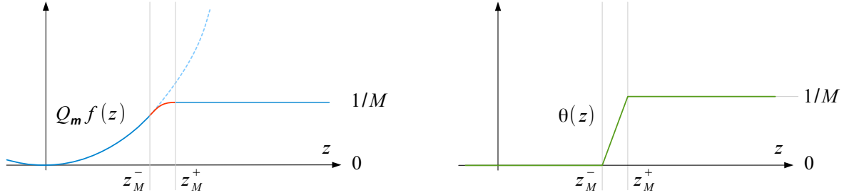
Figure 11: Q_{\mathbf{m}}f and \theta in a degenerate case.
