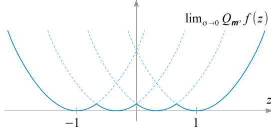
Figure 20: the limit of Q_{\mathbf{m}^\sigma} f for \sigma \rightarrow 0 in the case m_1 = 0 .
