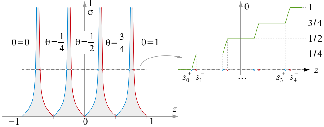
Figure 21: Representation of \theta in the z - \frac{1}{\sigma} plane for M = 4 (case m_1 = 0 )
