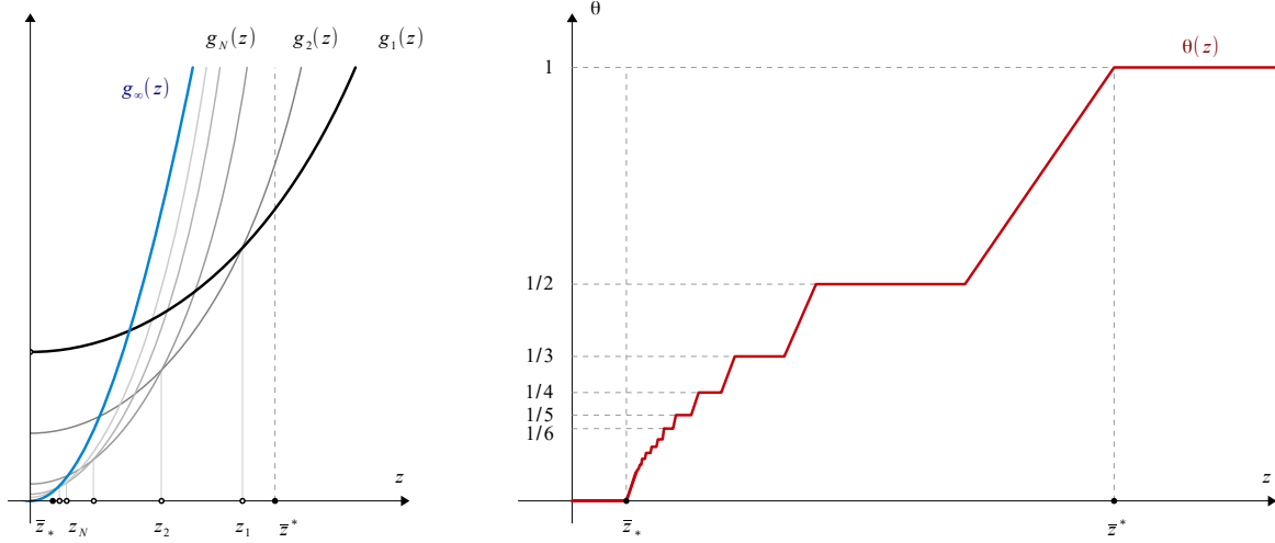
Figure 27: relative behaviour of g_N^\sigma and the final resulting \theta .
