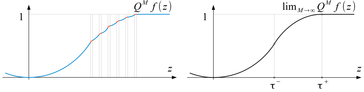
Figure 12: Graph of Q^M f(z) (for M = 6 ) and of the limit function.
