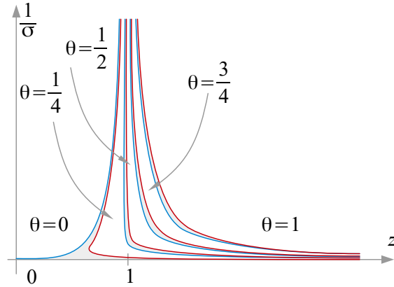
Figure 18: Representation of constancy sets of \theta in the z - \frac{1}{\sigma} plane ( M = 4 ).
