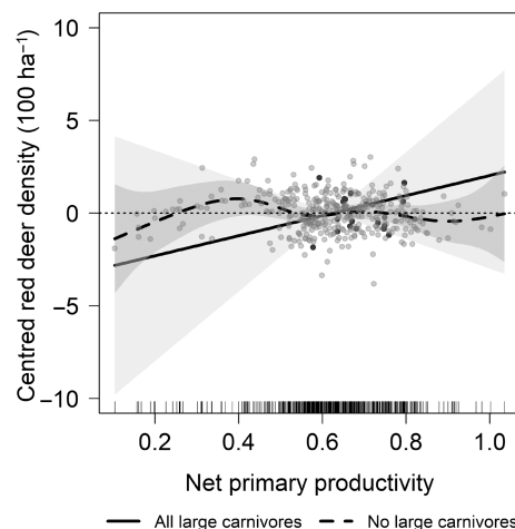
FIGURE 3 Plot of the generalized additive model predicting the effects of net primary productivity on red deer density (y-axis; log-scale) across Europe. Smooth functions were fit for sites with no large carnivores present (partial residuals; grey dots) and sites where all three carnivore species were present (partial residuals; black dots).
