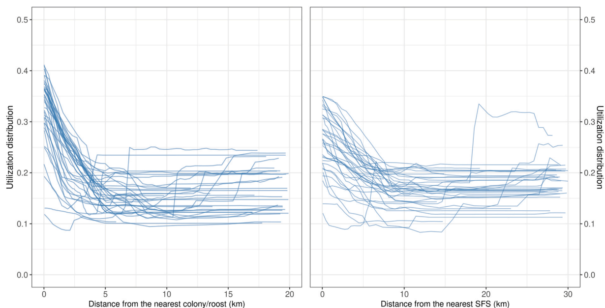
Fig. 3. Partial dependence plot of random forests, showing how the intensity of the occurrence distribution varied in function of the distance from roosts/colonies (panel on the left) and the distance from the nearest supplementary feeding stations (SFS, panel on the right).
