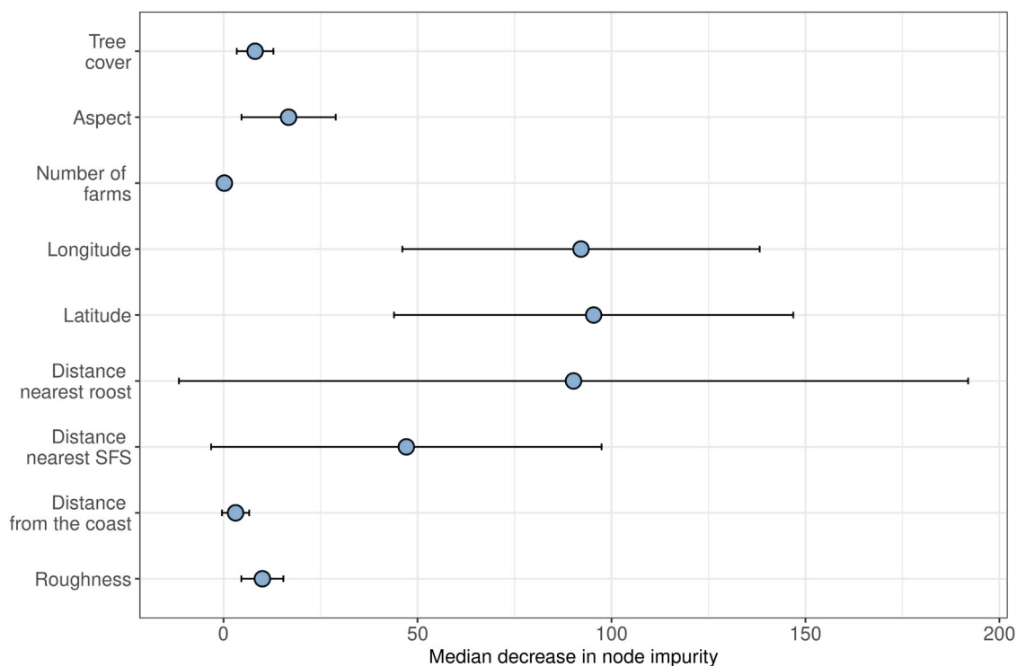
Fig. 2. Importance of the various predictors, expressed as the decrease in node impurities through the residual sum of squares. This value tells how well trees can split variables (the higher the better). Values were averaged for all 37 random forests: points represent median increase in node purity, and error bars standard deviation.
