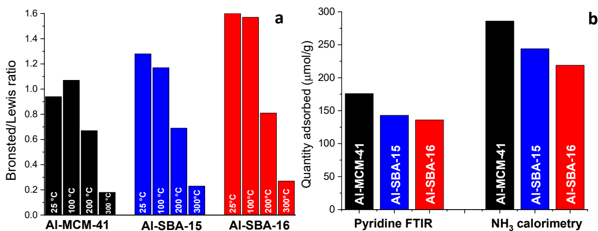
Figure 51 Brønsted/Lewis ratio determined on aluminosilicate samples with Py-FTIR at different temperatures (a). Comparison between the amount of total acid sites determined at 100 °C on aluminosilicate samples with Py-FTIR and the amount of irreversible acid sites determined with NH 3 adsorption calorimetry (b).
