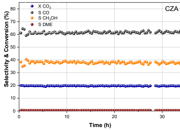
Figure 34. Conversion of CO 2 and selectivity to CO, methanol (MeOH) and dimethyl ether (DME) vs Time for the sample CZA [73].
