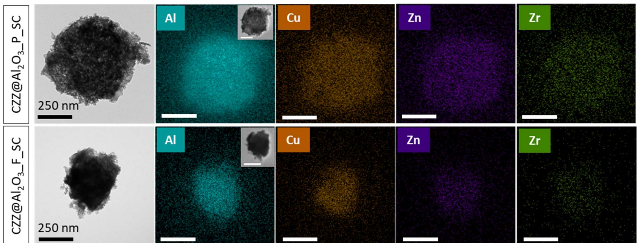
Figure 77 EDX chemical mapping of CZZ@Al 2 O 3 _P_SC (top row) and CZZ@Al 2 O 3 _F_SC (bottom row) composites [186].
