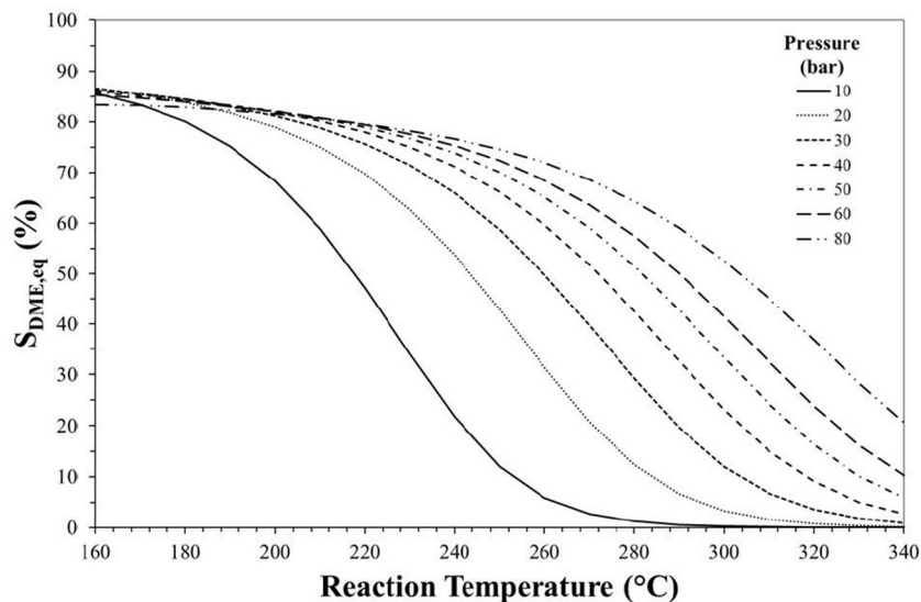
Figure 7 DME selectivity for the CO 2 -to-DME process at various temperatures and pressures. Reprinted from [15], distributed under the terms and conditions of the Creative Commons Attribution (CC BY) license.
