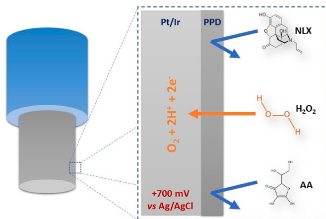
Fig. 1. Schematic representation of electrochemical assessments. Pt/Ir working electrode (cylinder) with an active surface of 1 mm and 125 \mu\text{m} Ø. Pt/Ir: Platinum/Iridium wire (90:10); PPD: polyorthophenylenediamine polymer.
