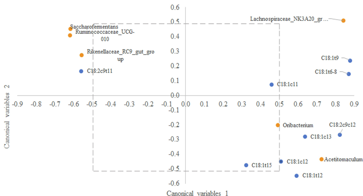
Fig. 2. Canonical correlation analysis (CCA) similarity maps for the bacterial genera and fatty acids involved in biohydrogenation (BHFA) in Maremma (A) and Aubrac (B).
