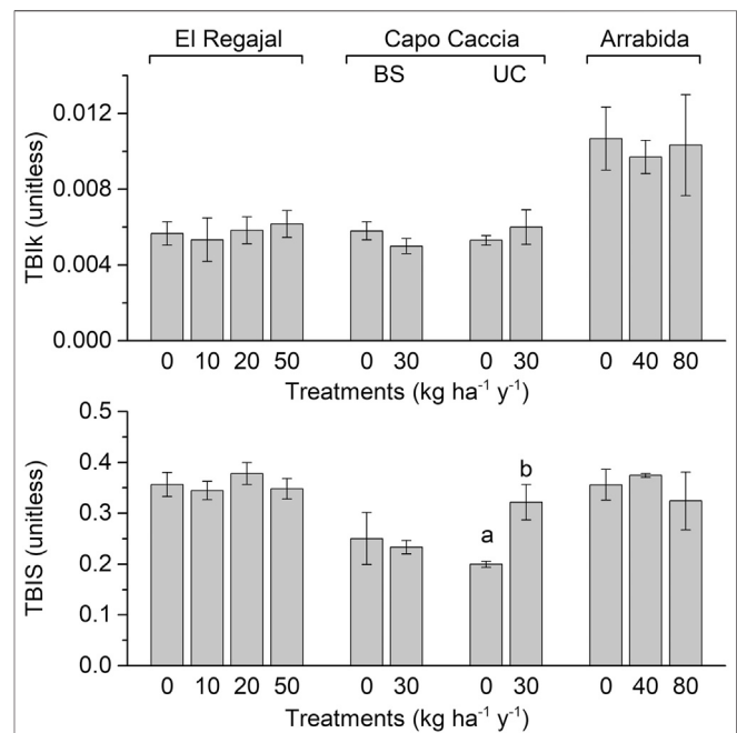
FIGURE 1 | Effect of nitrogen (N) addition on soil decomposition rate (TBlk) and stabilisation factor (TBIS) (means \pm SE) in the top 8 cm of the soil profile estimated through the tea bag index method for each N treatment in El Regajal (Spain, n = 6 ), Capo Caccia BS (Italy, n = 4 ), Capo Caccia UC (Italy, n = 4 ) and Arrábida (Portugal, n = 3 ). Capo Caccia BS and UC indicate bare soil and under canopy microsites, respectively. Tea bags incubations were performed for 65 days in spring 2014. Letters indicate significant differences among N treatments within each site ( p < 0.05 , one-way ANOVA, post hoc LSD test).
