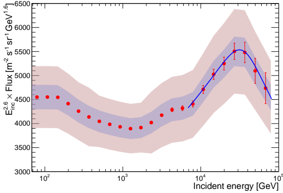
FIG. S10: Best-fit of the helium flux with a SBPL function (blue line) in the energy range [6.8 – 80] TeV, compared with the data. Error bars correspond to the statistical uncertainties, and the shaded bands show the systematic uncertainties.
