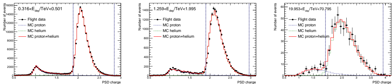
FIG. 1: The distributions of PSD charge, defined as the minimum charge value of the two PSD layers, for events with deposited energy ranges 316 – 501 GeV (left), 1259 – 1995 GeV (middle) and 19.95 – 70.79 TeV (right). The flight data are shown in black points. The histograms show the distributions of the best-fit proton MC (blue), helium MC (green), and proton + helium MC (red). The vertical dashed lines indicate the PSD charge range used to select helium candidate events.
