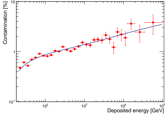
FIG. S6: Proton background percentage as a function of the BGO deposited energy. Solid line is a four-order polynomial fit, \sum_{i=0}^4 p_i \log^i(E_{\text{dep}}/\text{GeV}) .
