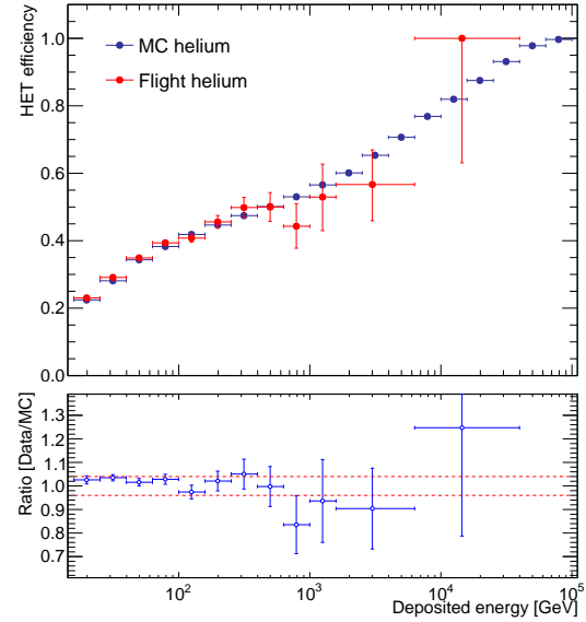
FIG. S2: The HET efficiencies as functions of the BGO deposited energy for the selected helium candidates of the flight data (red) and MC simulations (dark blue). The differences between the flight data and MC simulations are about 4% for energies up to 1 TeV.
