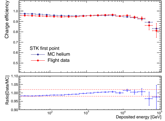
FIG. S5: Charge selection efficiencies for the first STK cluster point as functions of the BGO deposited energy. The differences between the flight data and MC simulations are about 2%.
