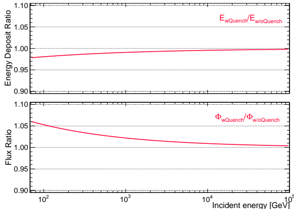
FIG. S7: The ratio of the quantities with the BGO quenching effect to that without the quenching effect. Top panel is for the mean energy deposition, and bottom panel is for the helium flux.
