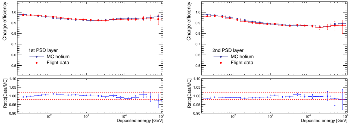
FIG. S4: Charge selection efficiencies for the two PSD layers as functions of the BGO deposited energy. The differences between the flight data and MC simulations are about 2% for both PSD layers.
