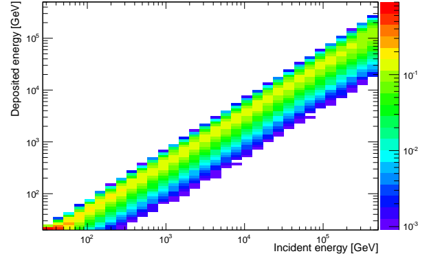
FIG. S8: Response matrix used in the unfolding procedure obtained from the selected MC helium sample.
