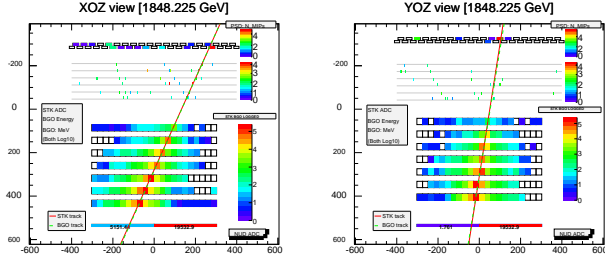
FIG. S1: Illustration of signals in all sub-detectors of DAMPE, for a candidate helium event with a raw energy of \sim 1.8 TeV.
