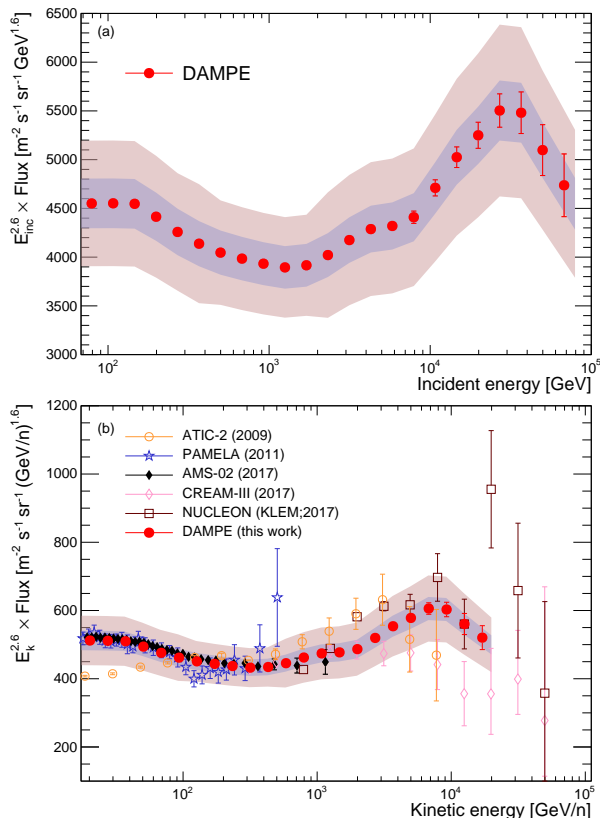
FIG. 3: Helium spectrum weighted by E^{2.6} (top panel) measured by DAMPE. In the bottom panel, we compare the DAMPE spectrum (converted to kinetic energy per nucleon assuming the AMS-02 measured {}^3\text{He}/{}^4\text{He} isotope ratio [26]) with previous measurements by PAMELA [4], AMS-02 [6], CREAM-III [3], ATIC-2 [2], and NUCLEON (KLEM) [9]. Error bars of the DAMPE data show the statistical uncertainties. The inner and outer shaded bands denote the systematic uncertainties from the analysis ( \sigma_{\text{ana}} ) and the total systematic uncertainties including those from hadronic models ( \sqrt{\sigma_{\text{ana}}^2 + \sigma_{\text{had}}^2} ). For the PAMELA and AMS-02 results, the error bars contain both the statistical and systematic uncertainties added in quadrature. For the other measurements, only the statistical uncertainties are shown.
