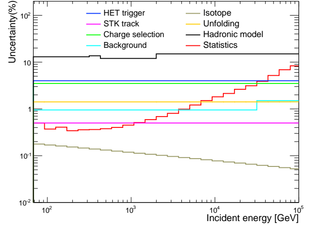
FIG. S9: Relative statistical and systematic uncertainties of the measured helium spectrum.
