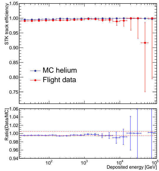
FIG. S3: The STK track efficiencies as functions of the BGO deposited energy. The differences between the selected helium candidates of the flight data and MC simulations are about 0.5%.
