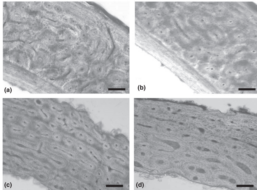
FIGURE 8 Histological sections of humerus (a) and ulna (b) of griffon vulture and humerus (c) and ulna (d) of flamingo
