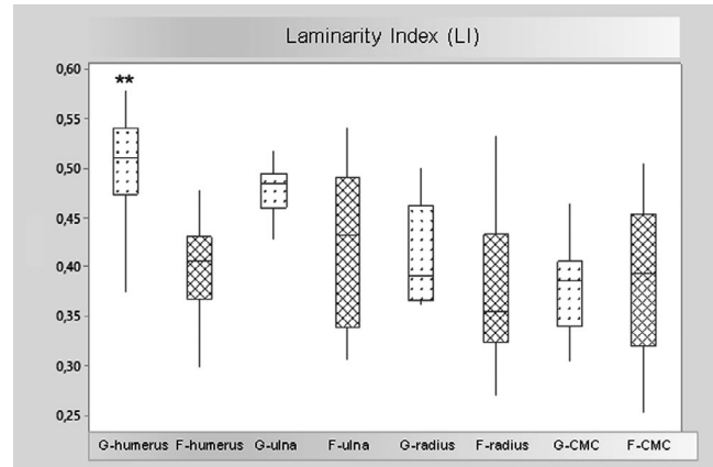
FIGURE 7 Laminarity index (LI) of the vascular canals in the bone tissue. G, griffon vulture; F, flamingo. ** p < 0.001
