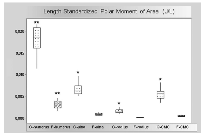
FIGURE 5 Length standardized polar moment of area (J/L). G, griffon vulture; F, flamingo. **p < 0.001 ; *p < 0.01
