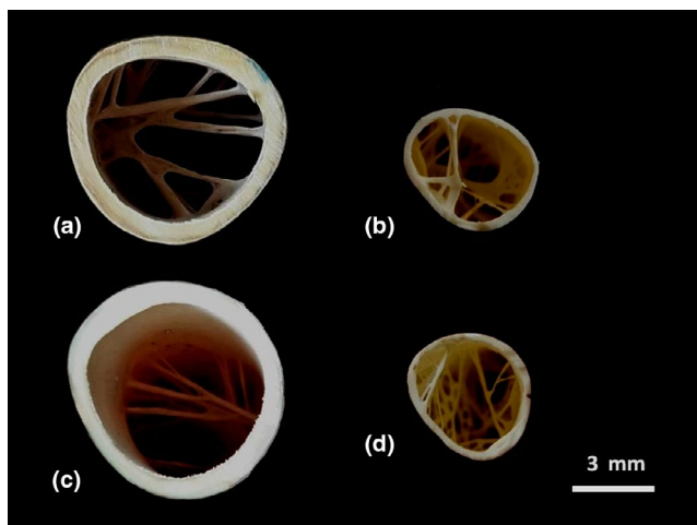
FIGURE 9 Transversal section of the humeri of griffon vulture (a, c) and flamingo (b, d). Humeri are the only pneumatized bones of the wing. Note the bone bridges crossing the diaphyseal cavity, which strengthen the whole bone during flight
