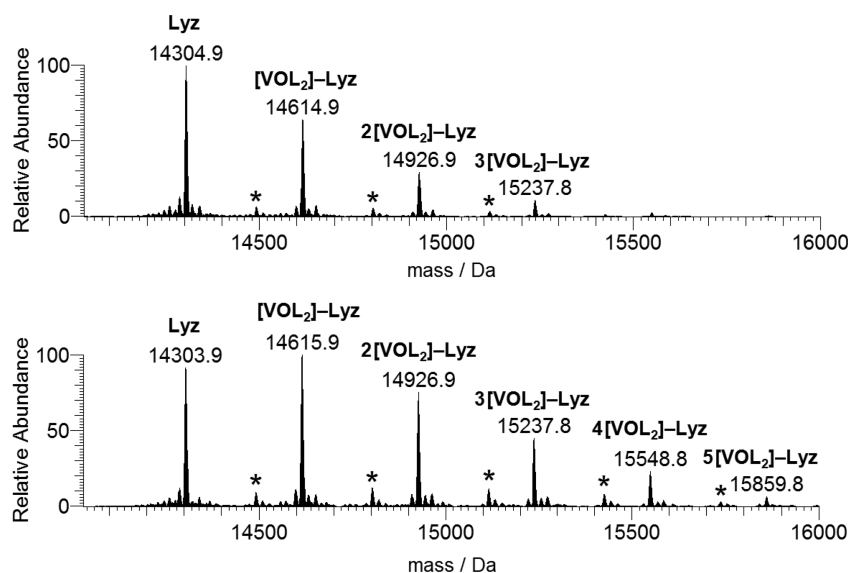
Figure 5. Deconvoluted ESI-MS spectra recorded on the system containing [\text{V}^{\text{IV}}\text{O}(\text{pic})_2(\text{H}_2\text{O})] and lysozyme ( 50\ \mu\text{M} ): molar ratios 3:1 (top) and 5:1 (bottom). L indicates the picolinato ligand. With the asterisks, the peaks of the adducts \{[\text{V}^{\text{IV}}\text{OL}]^+ + n[\text{V}^{\text{IV}}\text{OL}_2]^+\}-\text{Lyz} with n = 0-2 (ratio 3:1) and n = 0-4 (ratio 5:1) are denoted.
