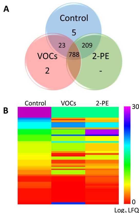
Fig. 2. Identified proteome dataset. The figure aims to provide a first introduction of the identified Aspergillus carbonarius MPVA566 proteomic dataset. Panel A depicts how the identified proteins are distributed along the three sample groups. The heatmap in panel B displays the protein dataset and, for each of the selected proteins, provides a visual impression of its abundance level, and how it changes in the diverse growing conditions. Protein abundance is expressed as \text{Log}_2 of LFQ abundance index.
