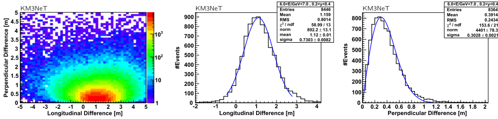
Figure 78. Longitudinal and perpendicular distance between the neutrino interaction position and the reconstructed vertex position for all selected events with E_\nu = 2 - 30 \text{ GeV} (left). Longitudinal distance for 6 \text{ GeV} < E_\nu < 7 \text{ GeV} and 0.2 < y < 0.4 fitted with a Gaussian (middle). Perpendicular distance for the same E_\nu and y range fitted with ‘distance \times a Gaussian’ (right).
