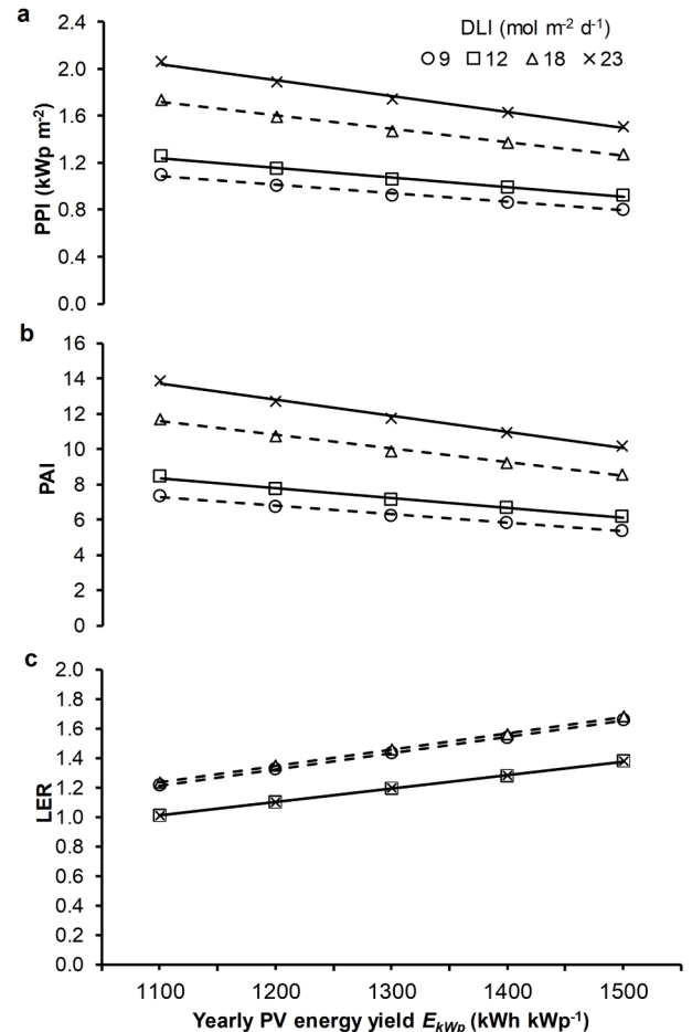
Fig. 7. PPI (a) and PAI (b) and LER (c) calculated in a energy self-sufficient scenario of the VFCA as a function of the PV energy yield and the DLI. All data is the average of the green leaf varieties.
