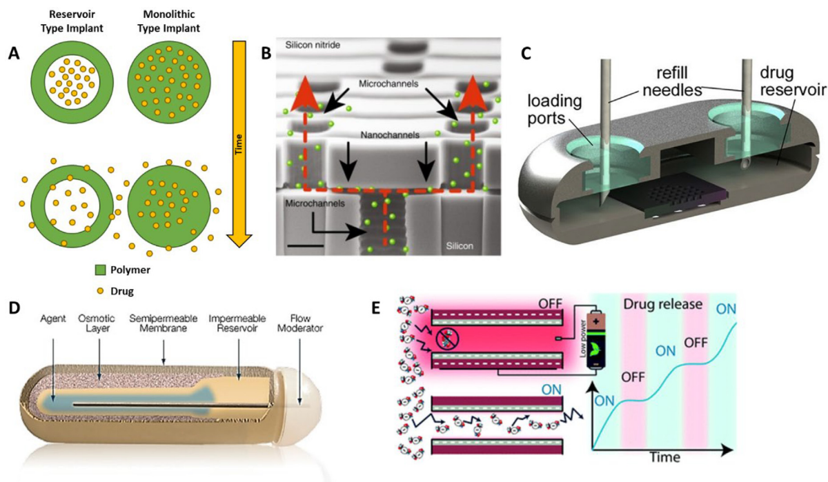
Fig. 2. Schematic of reservoir-type and monolithic-type implants (A). SEM image of a rate controlling membrane made of silicon containing micro- and nano-channels (scale bar: 1 \mu\text{m} ) (B). Diagram of a transcutaneous refillable implant (C). Diagram of ALZET® osmotic pump (D). Schematic of an electrostatically gated nanofluidic membrane (E). Reproduced with permission from DURECT Corporation, [21], [22] and [23].
