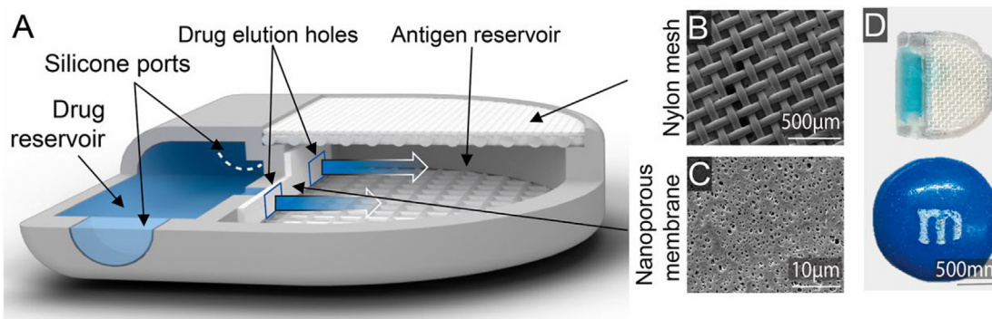
Fig. 12. Diagram showing NanoLymph structure (A). SEM images of the nylon mesh (B) and nanoporous membrane (C) used to limit the diffusion from the reservoirs. Image showing the size of the implant next to a commercial M&M (D). Scale bar: 500 \mu m. . Reproduced with permission from: [391]
