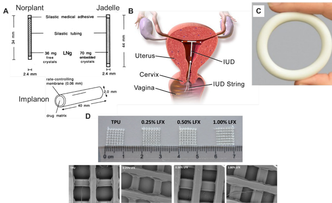
Fig. 3. Diagrams showing the structure of several subdermal contraceptive implants (A), diagram showing an implanted intrauterine device (B). Image of Annovera® Intravaginal Ring (C). Pictures and SEM images of 3D printed meshes containing different levofloxacin loadings (D). . Reproduced with permission from: [119,141,145,146]
