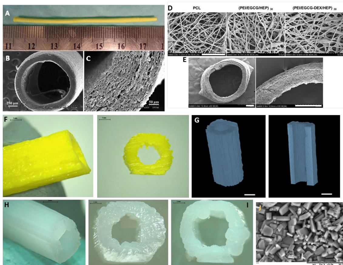
Fig. 9. A macroscopic view of the electrospun DIP-eluting SDVG (A) and its electronic cross-section images (B and C). Scanning electron microscope (SEM) images of the electrospun PCL-based SDVGs before and after modification (D) and their cross-sections (E). Scale bars were 10 and 500 \mu\text{m} , respectively. PCL-based 3D-printed SDVGs containing 20% DIP (F), and images of the performed X-ray microcomputed tomography in this study, indicating a homogeneous structure was obtained. (G). PCL-based 3D printed SDVGs with no drug (H) and containing 10% ASA (I), and a SEM image of the surface of the last SDVGs containing 10% ASA (J). Reproduced with permission from the cited references [107,259,262,306].
