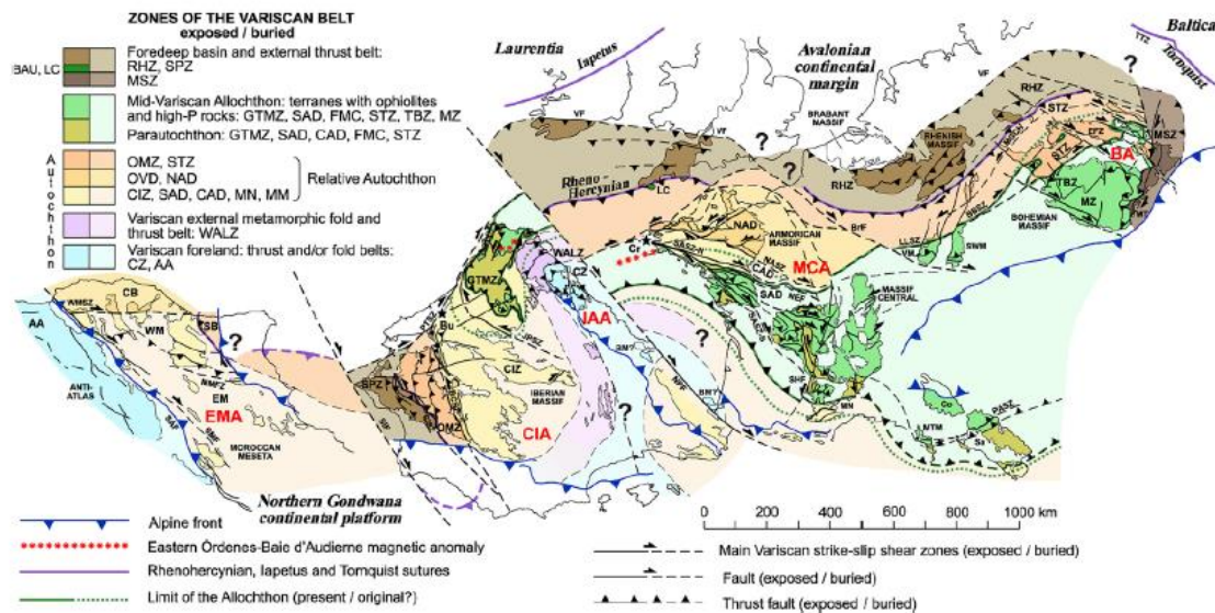
Fig. 1 Tectonic sketch map of the Southern Variscan Realm at the end of the Paleozoic (after Martínez Catalán et al. 2021). Zones (Z): CZ Cantabrian, CIZ Central Iberian (OVD, Obejo-Valsequillo Domain), GTMZ Galicia-Trás-os-Montes, MSZ Moravo-Silesian, MZ Moldanubian, OMZ Ossa-Morena, RHZ Rhenohercynian, SPZ South Portuguese, STZ Saxo-Thuringian, TBZ Teplá-Barrandian, WALZ West Asturian-Leonese. Armorican Domains (AD): CAD Central, NAD North, SAD South, MM Moroccan Meseta (AA, Anti-Atlas; CB, Coastal Block; EM, Eastern Meseta; SB, Sehoul Block; WM, Western Meseta). Shear zones (SZ), faults (F) and fault zones (FZ): BBSZ Baden-Baden, BCSZ Badajoz-Córdoba, BrF Bray, EFZ Elbe, JPSZ Juzbad-Penalva, LLSZ Lalaye-Lubine, MMFZ Middle Meseta, MT Moldan-
