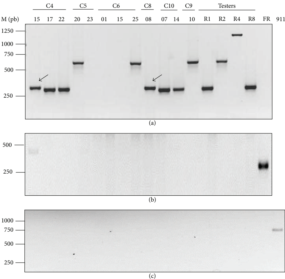
FIGURE 4: Specific Fod-race primers showing different amplification products. Agarose gel electrophoresis (1.5%) of PCR products from the genomic DNA of 12 representative RAPD group isolates, four Fod testers, and one Fusarium redolens isolate. (a) Multiplex PCR in which five primers were mixed in the same reaction tube, where combinations of Ft3/R8.1, Ft3/R2.1, and Ft3/R4.2 resulted in bands of 295 (race 1/8), 564 (race 2), and 1315 bp (race 4), respectively; bands with retarded electrophoretic mobility are shown with an arrow. (b) Multiplex PCR products obtained with the LSU (not shown) and Fusarium redolens -specific primers, with a resulting band of 386 bp. (c) PCR of the eubacterial primers 704f and 1495r where a 900 bp product was not amplified. Fod testers R1 (race 1), R2 (race 2), R4 (race 4), and R8 (race 8); Fr: Fusarium redolens and 911 (bacterial tester). M: molecular size marker (1 kb ladder, Biotools); sizes (base pairs) are indicated on the left.
