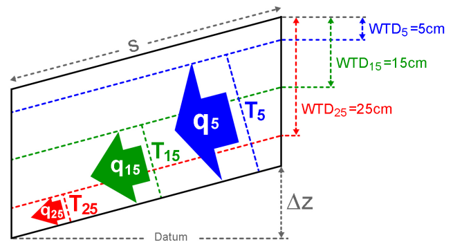
Figure 1. Schematic diagram of a drainage experiment carried out on a soil block. Measured flows per unit width of the block ( q_{\text{WTD}} ) and thickness of the flow zones ( T_{\text{WTD}} ) for different water table depths (WTDs), distances along the sloping bed ( s ), and water table elevation from an arbitrary datum ( \Delta Z ).
