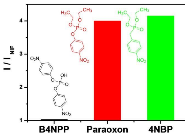
Figure 8. Bar plot showing the selectivity of molecularly imprinted film material towards solutions of bis(4-nitrophenyl) phosphate, diethyl(4-nitrobenzyl)phosphonate and paraoxon (for 1349 \text{cm}^{-1} Raman mode) with respect to not-imprinted film (normalised to 1).
