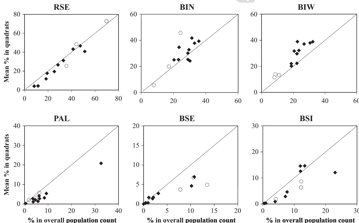
Fig. 7. Mean frequency of each floral type in mixed populations of Cyclamen balearicum and C. repandum subsp. repandum on Corsica (white symbols) and Sardinia (black symbols). The y-axis represents the mean frequency of a given floral type in the 1-m 2 plots and the x-axis depicts the frequency of the floral type in the random population count. The black line represents the bisector (equal frequency in the two types of count). RSE – large pink flowers typical of Cyclamen repandum subsp. repandum , bicoloured flowers with a wide (BIW) or narrow (BIN) basal ring (grey bars), PAL – pale-pink flowers and white flowers with an exerted (BSE) or inserted (BSI) stigma (white bars).
