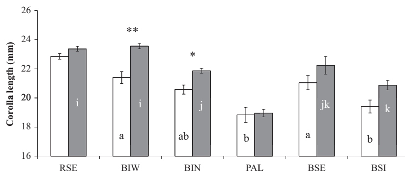
Fig. 6. Comparison of corolla length of the six floral types in mixed populations of Cyclamen balearicum and C. repandum subsp. repandum on Corsica (white bars) and Sardinia (black bars). Stars indicate significant differences between islands for a given floral type. A common letter in different bars means no significant difference (see Table 2).
