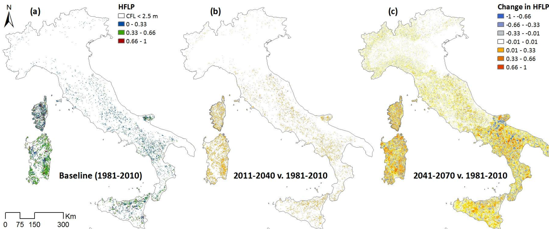
Fig. 9. Maps of High Flame Length Probability (HFLP), which is the probability of high flame length (> 2.5 m) given a fire burning the cell: for the baseline period (1981-2010) (a); difference between first future period (2011-2040) and baseline (b); and difference between second future period (2041-2070) and baseline.
