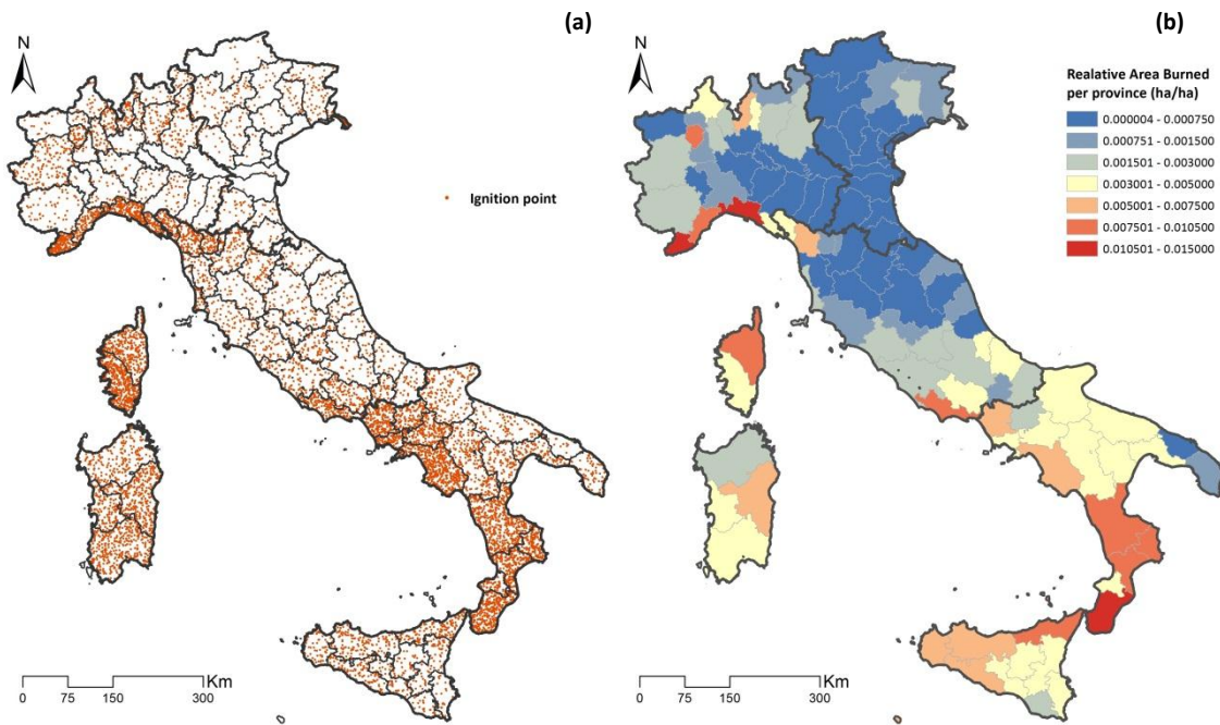
Fig. 3. Average annual fire ignitions at province level (a) and annual area burned relative to the area covered by each province (ha/ha) (b) from historical data (fires occurred from 1990 to 2008, source: JRC).
