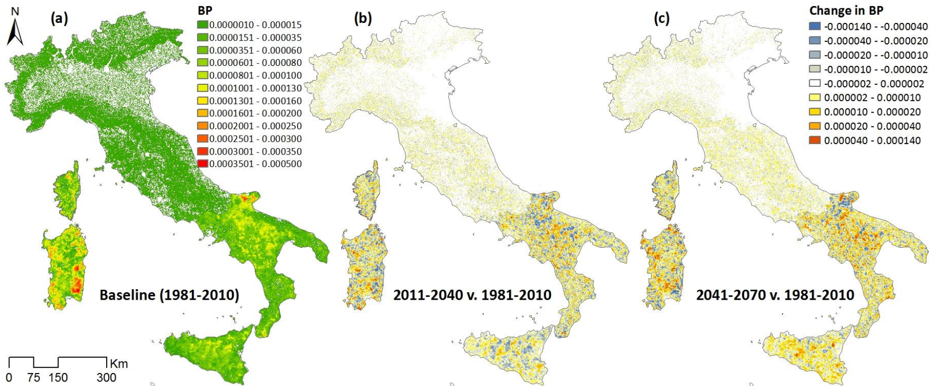
Fig. 5. Maps of Burn Probability (BP): for the baseline period (1981-2010) (a); difference between first future period (2011-2040) and baseline (b); and difference between second future period (2041-2070) and baseline.
