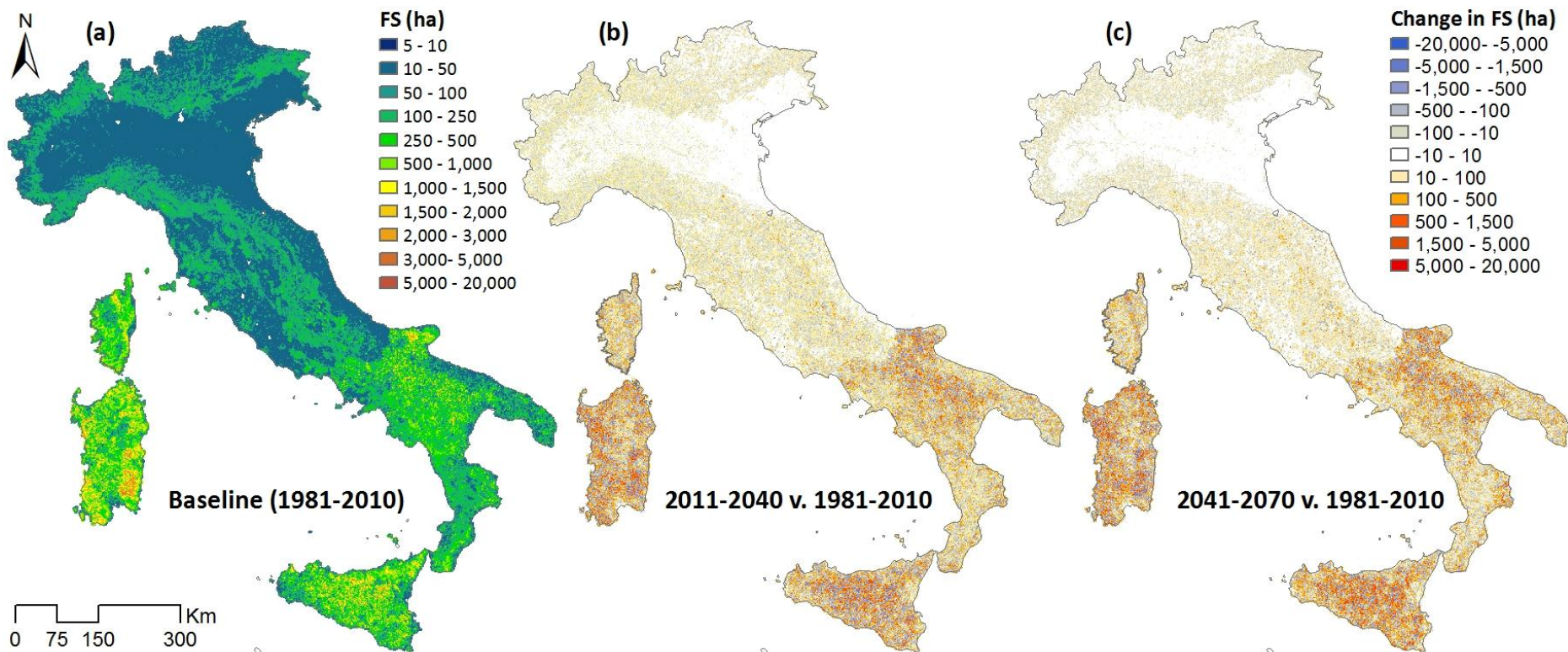
Fig. 7. Maps of Fire Size (FS): for the baseline period (1981-2010) (a); difference between first future period (2011-2040) and baseline (b); and difference between second future period (2041-2070) and baseline.
