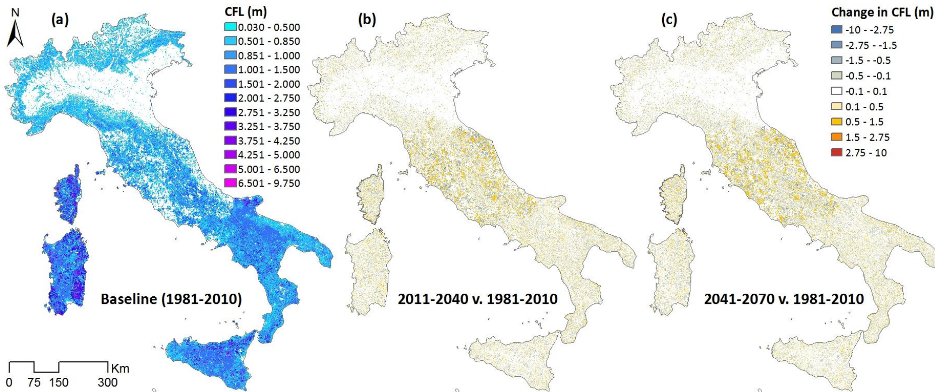
Fig. 6. Maps of Conditional Flame Length (CFL): for the baseline period (1981-2010) (a); difference between first future period (2011-2040) and baseline (b); and difference between second future period (2041-2070) and baseline.
